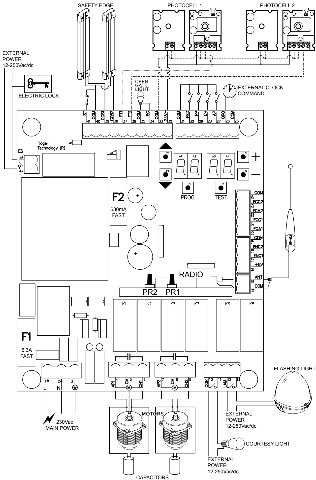
FIGURE 1 ELECTRICAL CONNECTIONS
