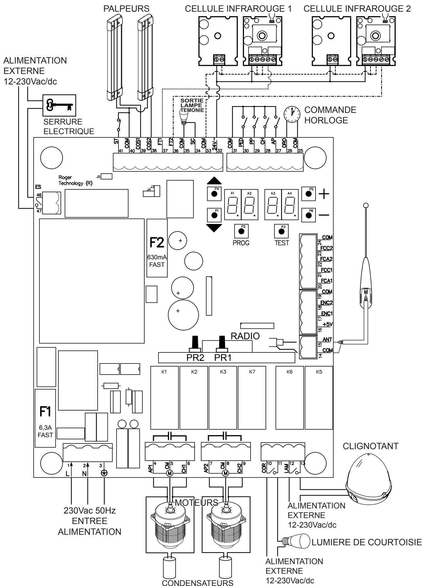
FIGURE 1 BRANCHEMENTS AUX BORNES
